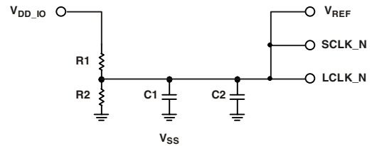
R1: 2k \Omega SERIES RESISTOR R2: 1.67k \Omega SERIES RESISTOR C1: 1 \mu F CAPACITOR (SMD) C2: 1nF CAPACITOR (HF SMD) PLACED CLOSE TO DSP'S PINS
