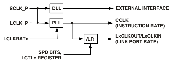
Figure 5. Clock Domains
