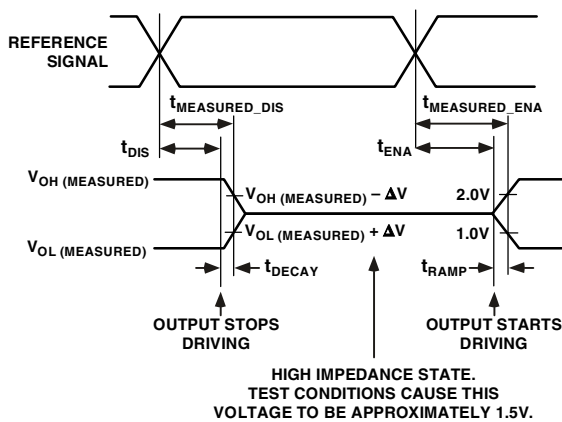
Figure 29. Output Enable/Disable
