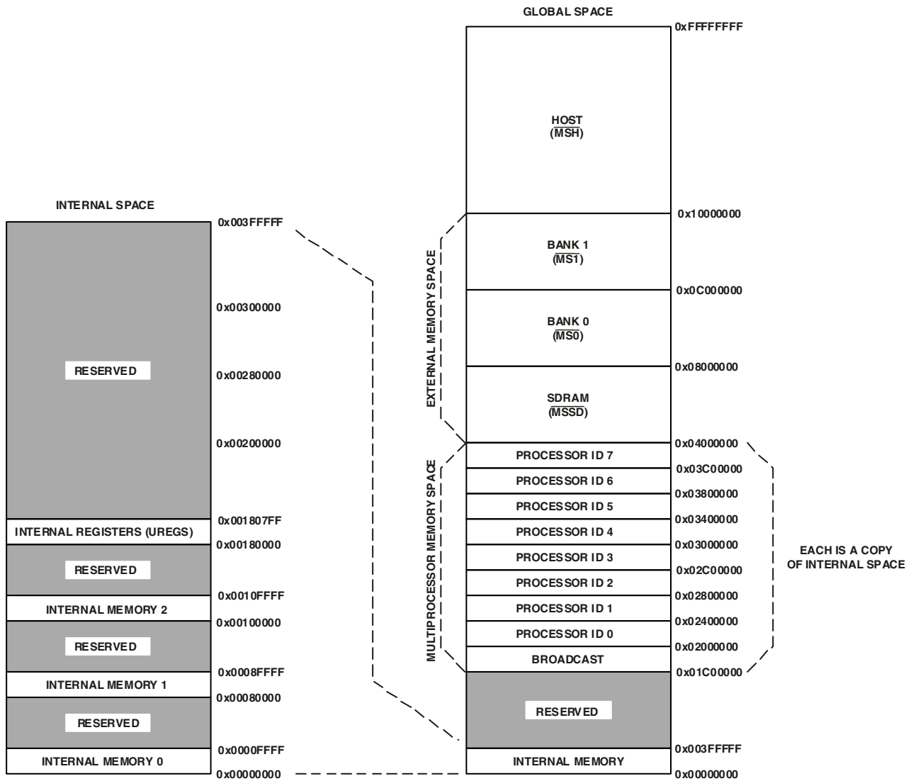
Figure 3. Memory Map
